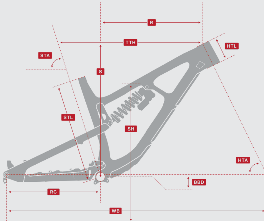
Slayer 29"
